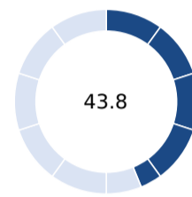
Strength of insolvency framework index
